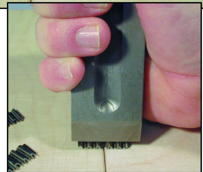
Corrugated fastener insertion tool holds fasteners securely and keeps fingers away from head of hammer.
