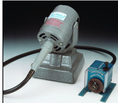
Quicknick Grinder - 110 V version.
